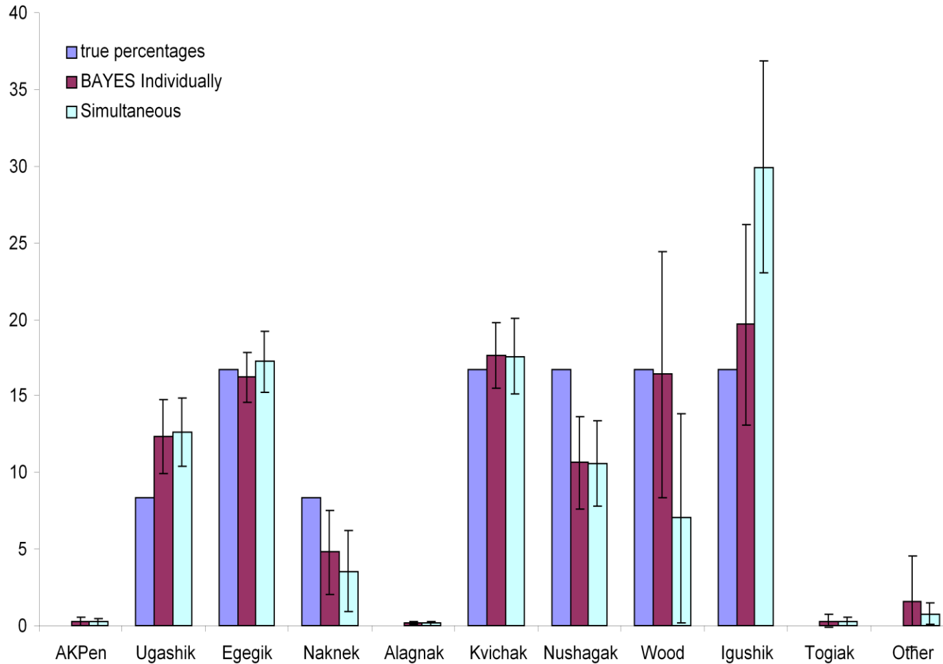
Figure 1. Stock composition estimates and standard deviations for 10 mixtures made up of 240 sockeye salmon each. Each mixture contained fish taken from the escapement of rivers in the same proportions (“true percentages”). Two methods for estimating stock proportions were used: 1) the standard one-mixture-at-a-time method (“BAYES Individually”) and, 2) a method that used the information from all the mixtures simultaneously in the baseline (“Simultaneous”).
